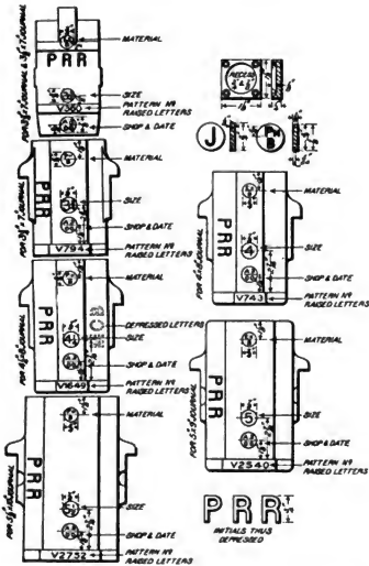
Figs. 4782-4794. Standard Markings for Journal Bearings. (439)
